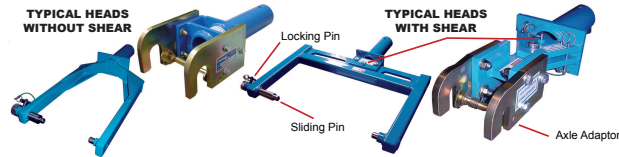
TYPICAL MULTI-HEAD TOWBAR
