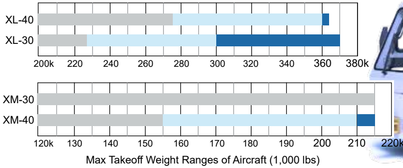
Eagle XL and XM Series - Safe Handling Chart
